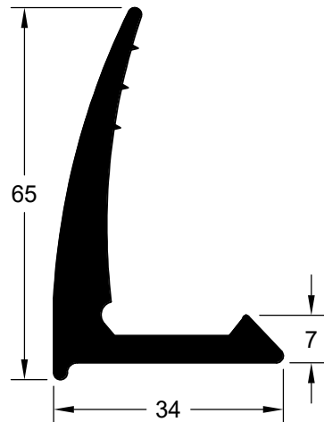
CIA 9144 (EPDM 70 Shore A)
