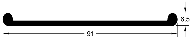
CIA 6237 (EPDM 80 Shore A) CIA 16801 (TPE 70 Shore A)
