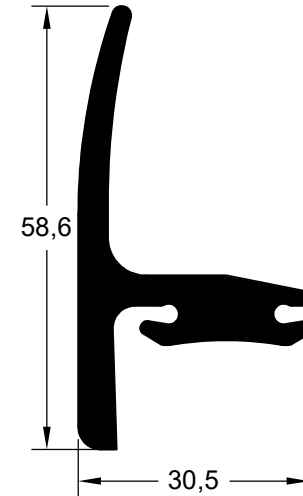
CIA 18017 (EPDM 80 Shore A)
