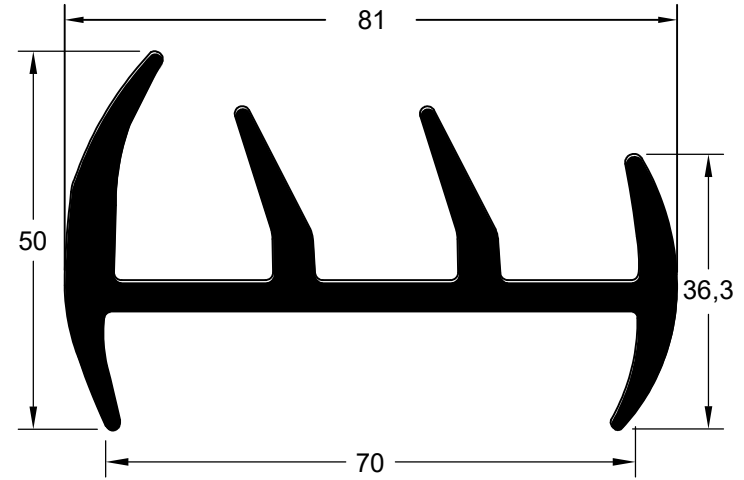
CIA 18479 (EPDM 75 Shore A)
