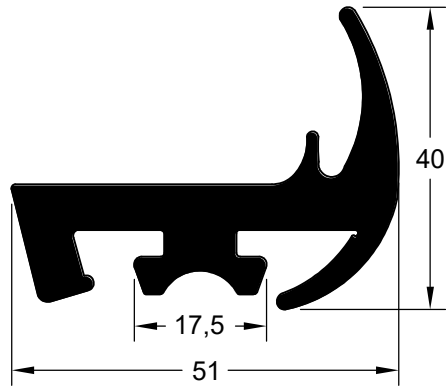
CIA 7029 (TPE 70 Shore A)
