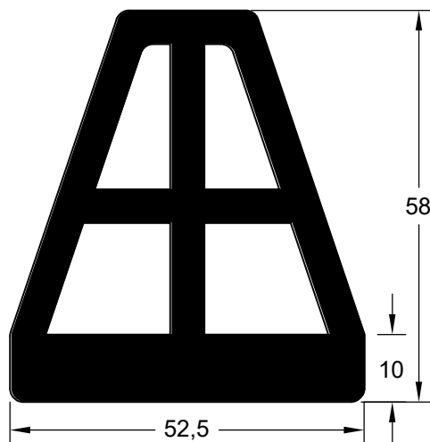
CIA 6341 (EPDM 80 Shore A)
