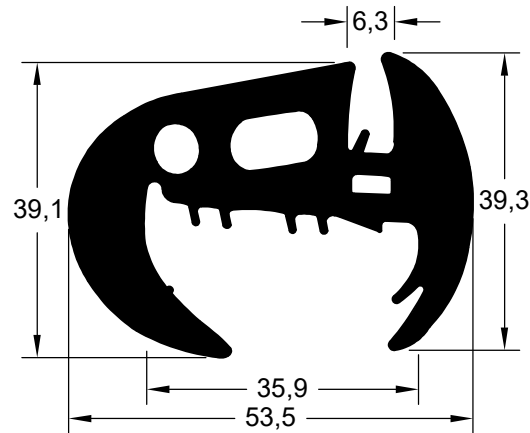
CIA 18648 (EPDM 63 Shore A)
