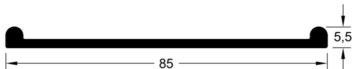
CIA 6352 (EPDM 70 Shore A) CIA 16564 (TPE 70 Shore A)
