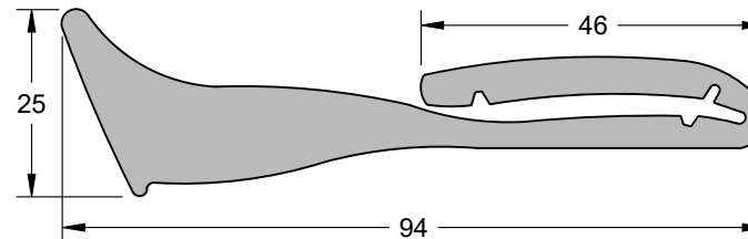
CIA 4160 (SBR 15 Shore A)
