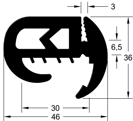
CIA 9153 (EPDM 63 Shore A)
