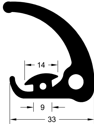
CIA 9144 (EPDM 70 Shore A)
